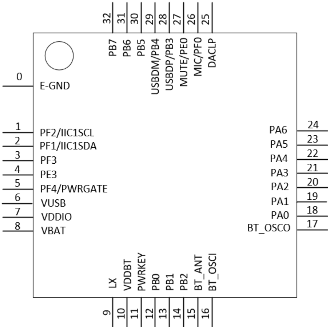
Figure 3-1 AB5682C Pin assignment for QFN32 4x4
