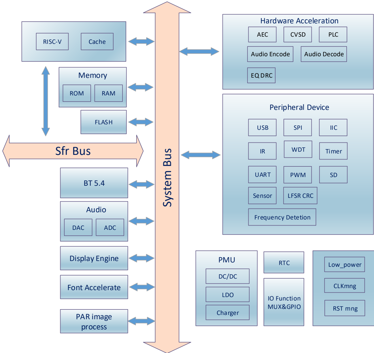
Figure 2-1 Soc Architecture Block Diagram
